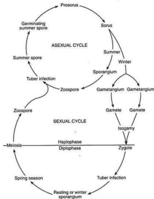
Fig. Schematic representation of life cycle of S. endobioticum
