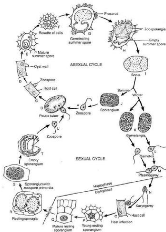
Fig. Life cycle of Synchytrium endobioticum
